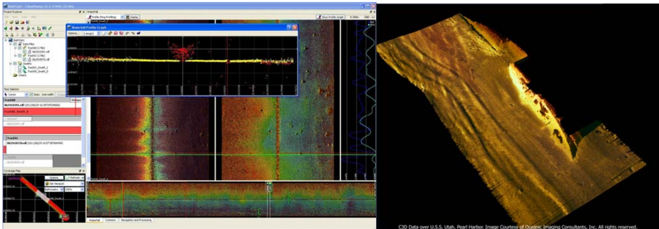
Left - Batch-interactive data processing screen in CleanSweep3, showing some of the the simultaneous interactive displays and the global cursor. Data: Teledyne-Gavia, Image: Thurne Hydrographic Ltd. Right - USS Utah, Pearl Harbor. Bathymetry and co-registered side scan data from a Teledyne-Benthos C3D survey, data processed in CleanSweep3. Image: OIC inc.
