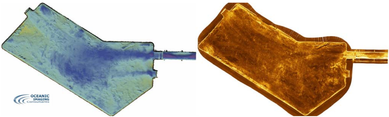
Interferometric bathymetry (0.5m grid) and sidescan (0.2m mosaic) of Chatham Docks, London, UK, from a 500kHz GeoSwath plus survey processed using CleanSweep3 software. Note the returns from under the docked vessels (the hull outlines on the north quay are visible in the sidescan image). Data: Peel Ports Medway, Images: OIC inc.
