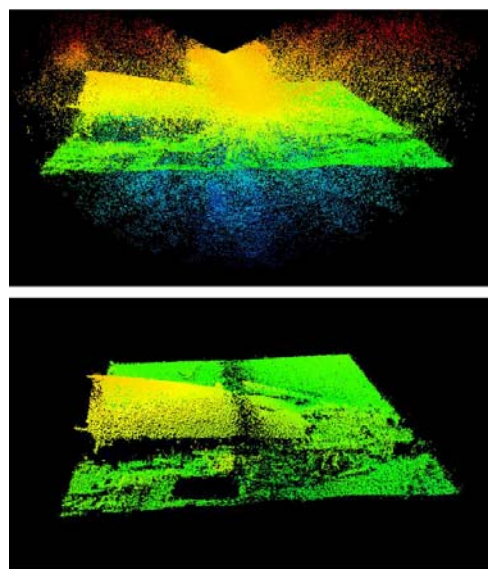
A typical Interferometric data cloud from a few seconds of survey, before (top) and after (bottom) processing. Data from an AUV survey over a wreck and debris field, 80m swath width. Processed using filters designed for interferometric data in CleanSweep3. Data: Teledyne-Gavia, image: OIC Inc.
